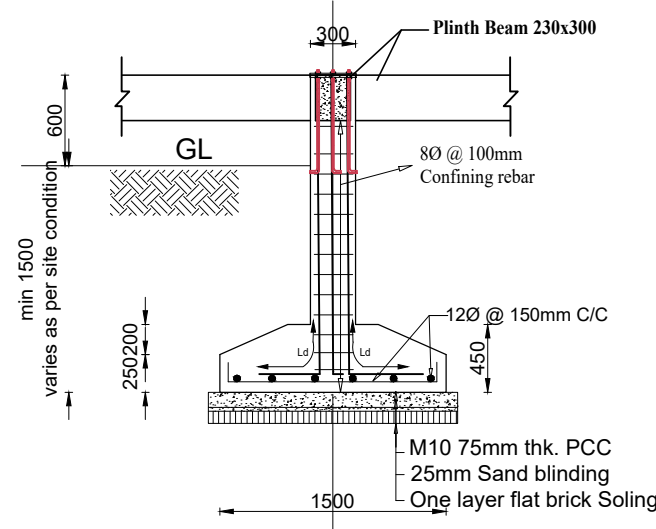
TYPICAL COLUMN PROFILE (300x300) SCALE=1:50
