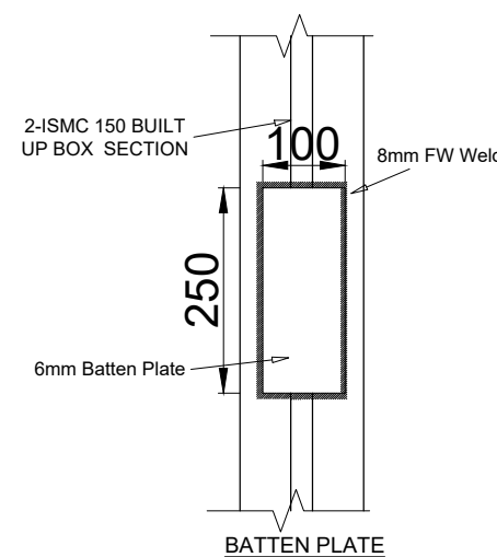
BATTEN PLATE
