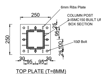
TOP PLATE (T=8MM)
