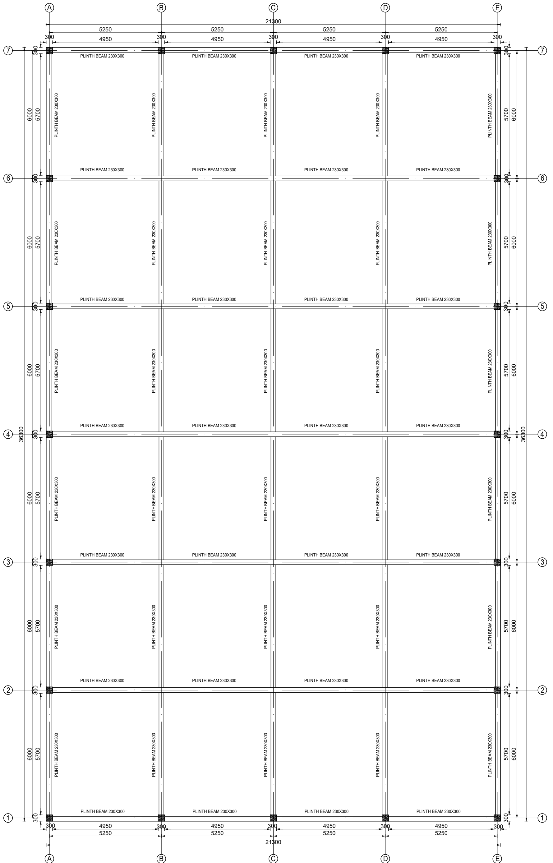
PLINTH TIE BEAM PLAN SCALE=1:100
