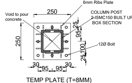
TEMP PLATE (T=8MM)
