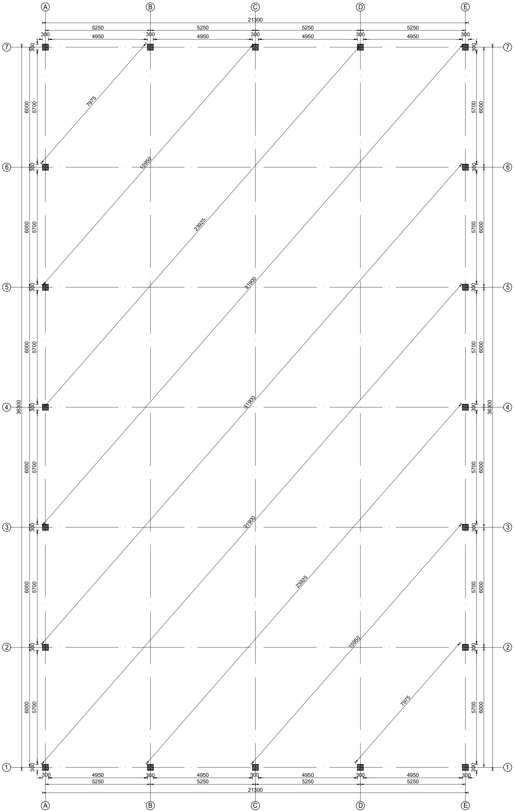
RCC COLUMN LAYOUT PLAN SCALE=1:100
