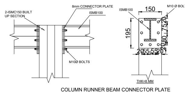
COLUMN RUNNER BEAM CONNECTOR PLATE
