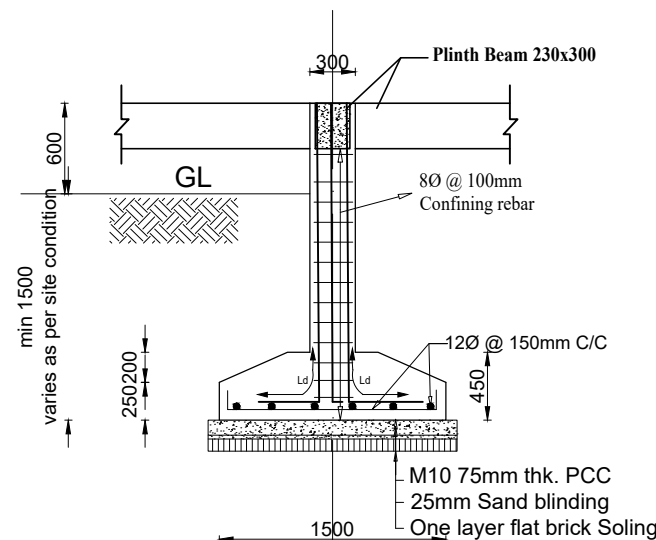
ISOLATED FOOTING SECTION SCALE=1:50
