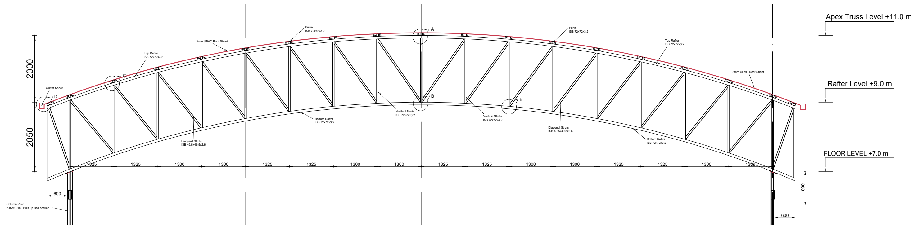
TRUSS PROFILE 2 SCALE=1:50
