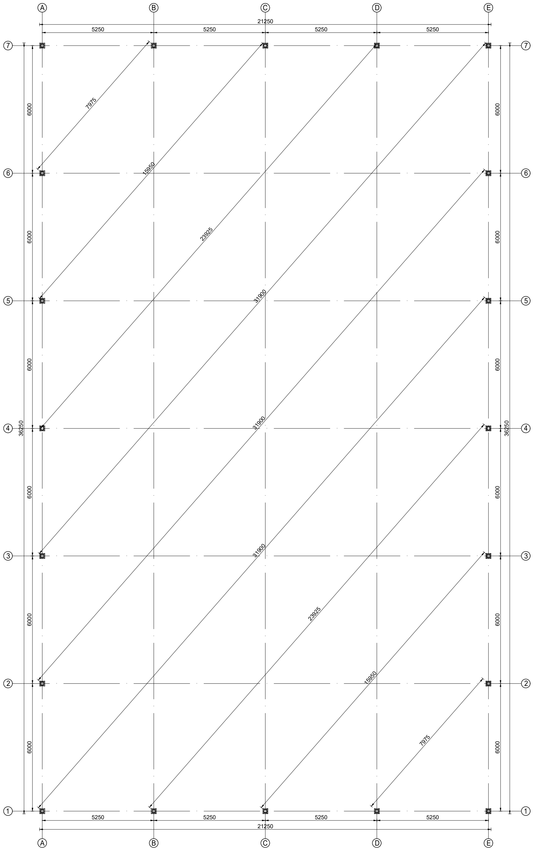
STEEL COLUMN PLAN (2-ISM 150 BUILT UP SECTION) SCALE=1:100
