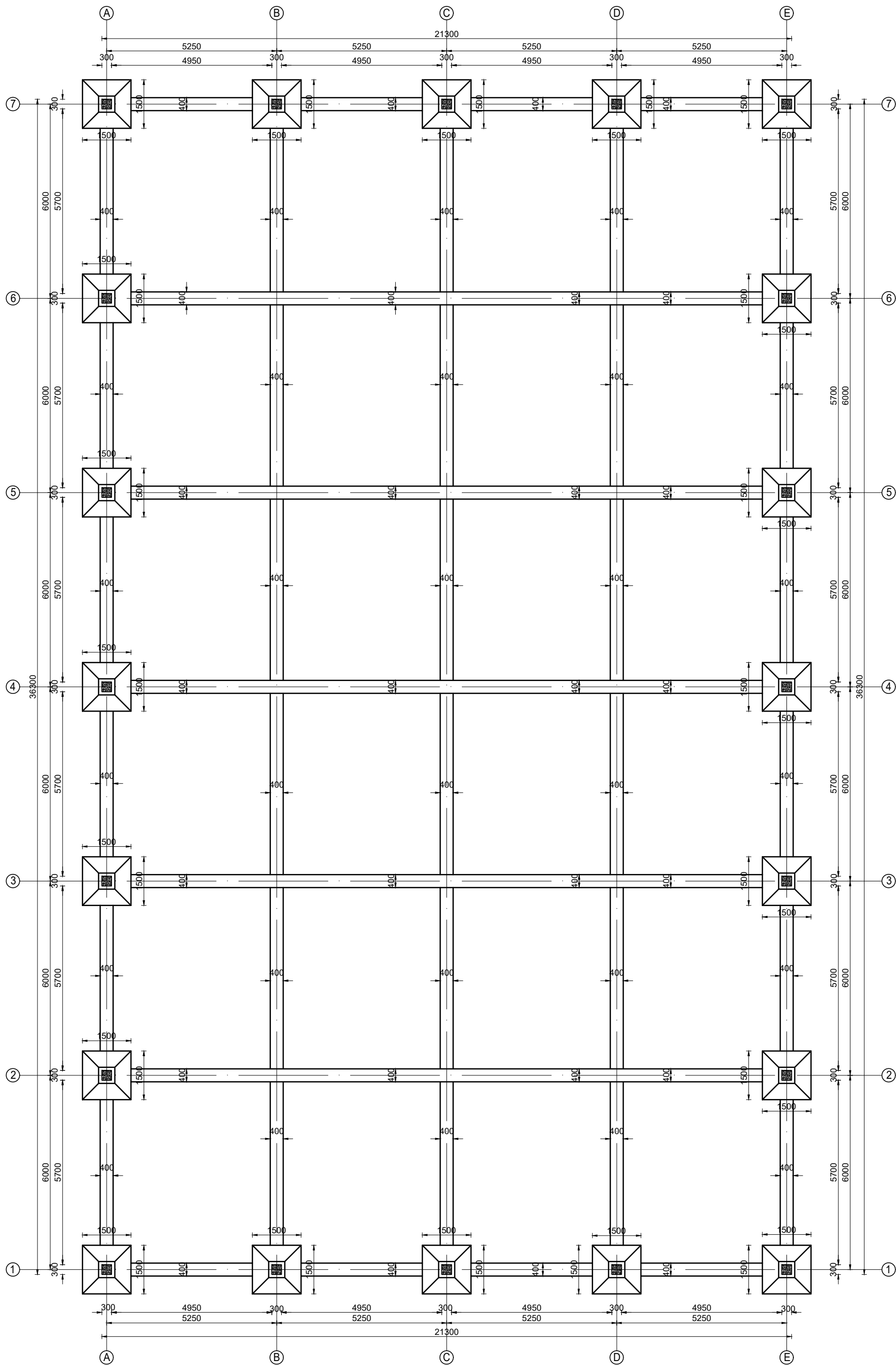
TRENCH AND FOUNDATION PLAN
