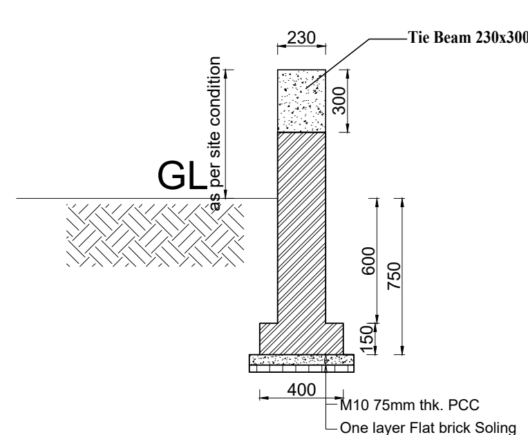
TYPICAL TOE WALL SECTION SCALE=1:25
