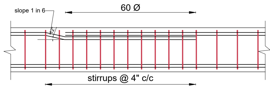
LAPPING DETAIL AT Y
