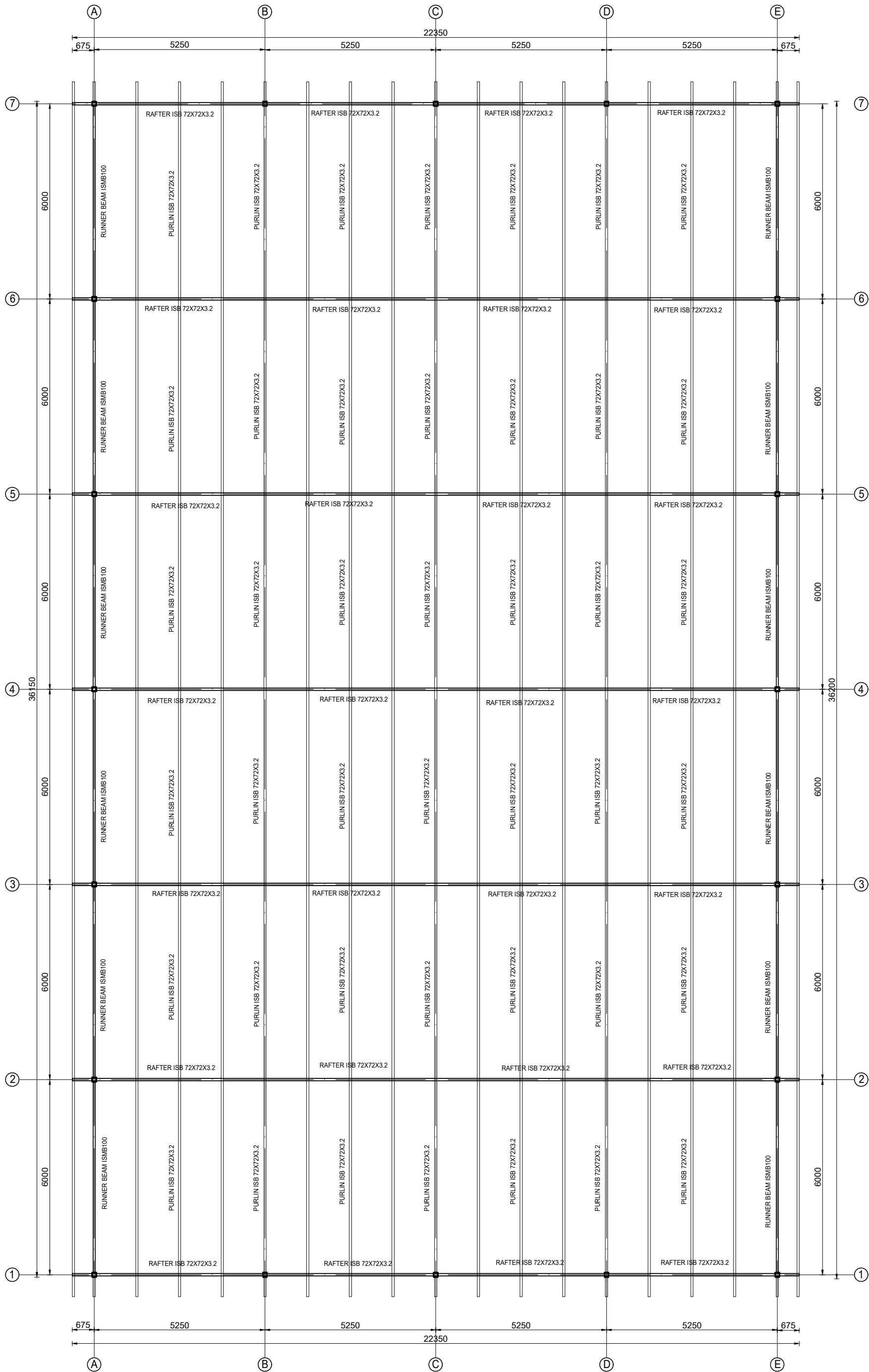
TRUSS AND RUNNER BEAM PLAN SCALE=1:100
