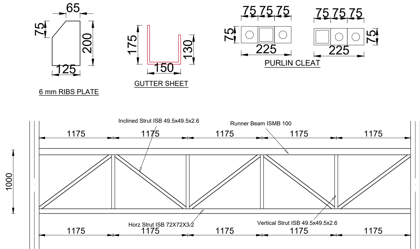
GIRDER BEAM 1 BRACING DETAIL SCALE = 1:50
