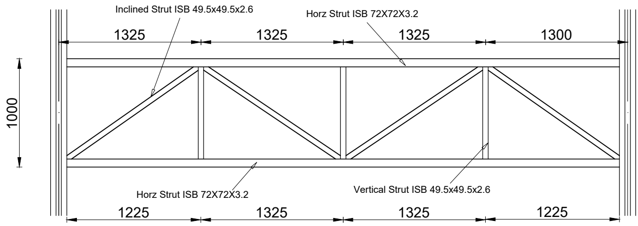
GIRDER BEAM 2 BRACING DETAIL SCALE = 1:50
