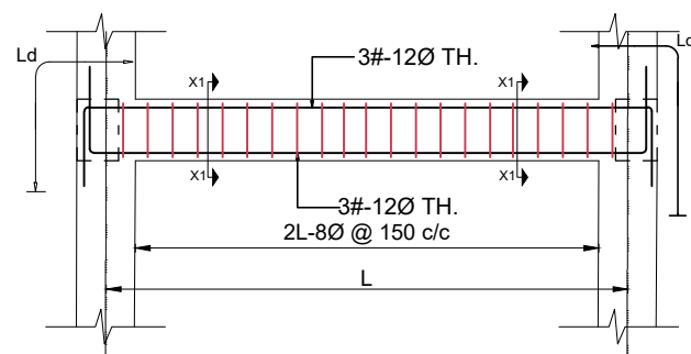
PLINTH TIE BEAM PROFILE Scale= 1:50
