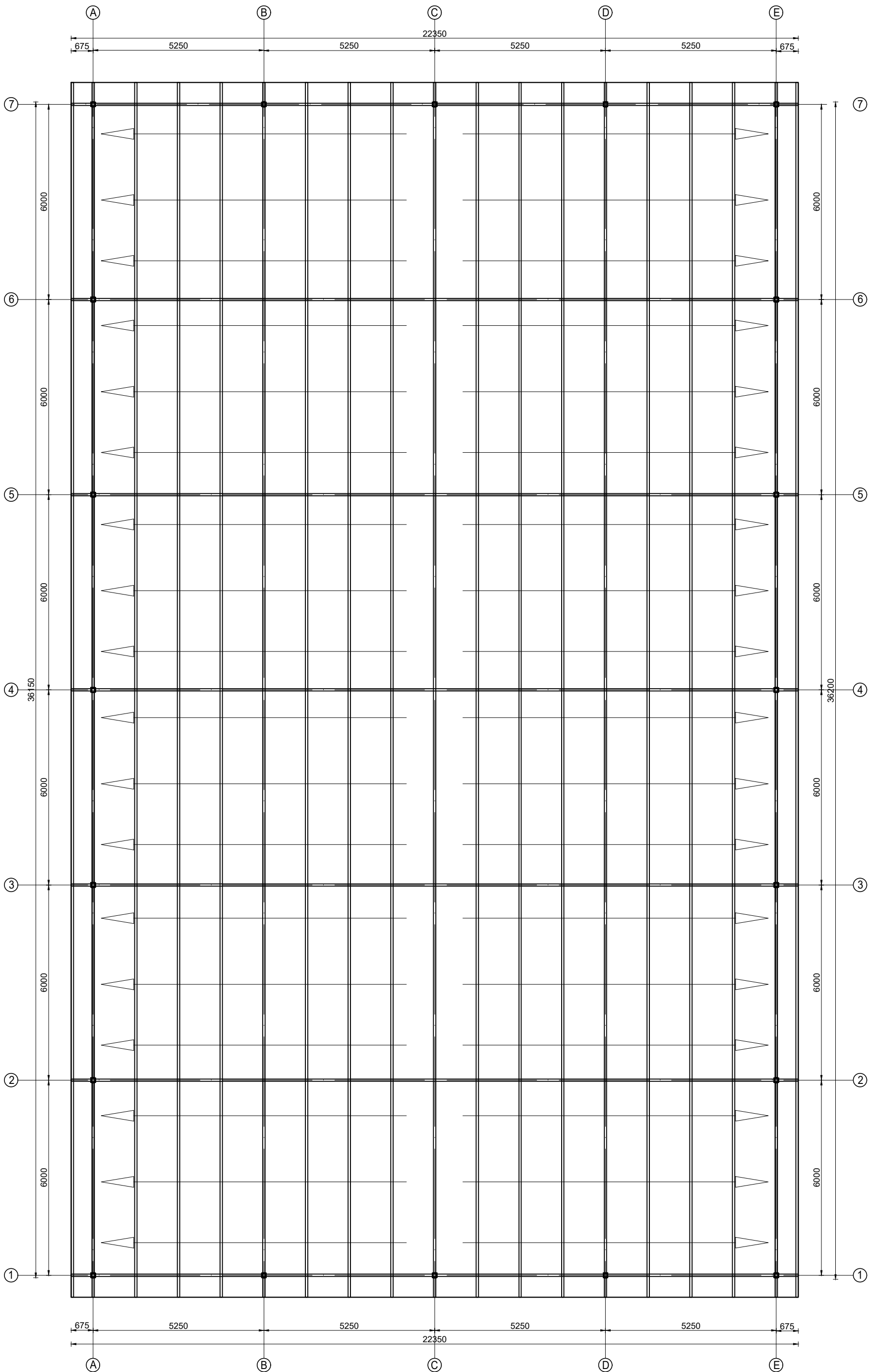
ROOF PLAN (3mm UPVC ROOFING SHEET) SCALE=1:100
