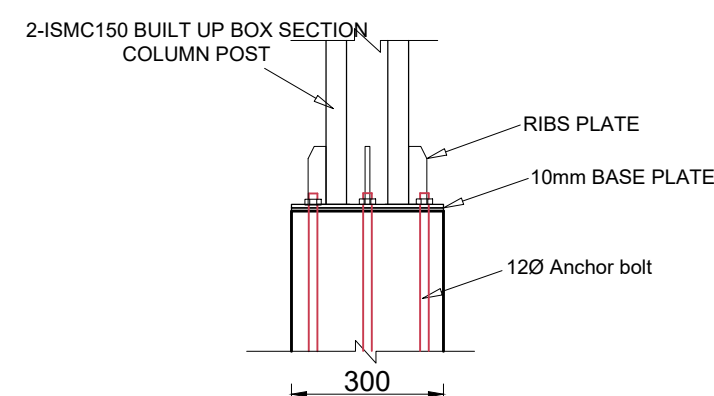
STEEL RCC COLUMN CONNECTION
