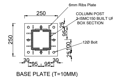
BASE PLATE (T=10MM)
