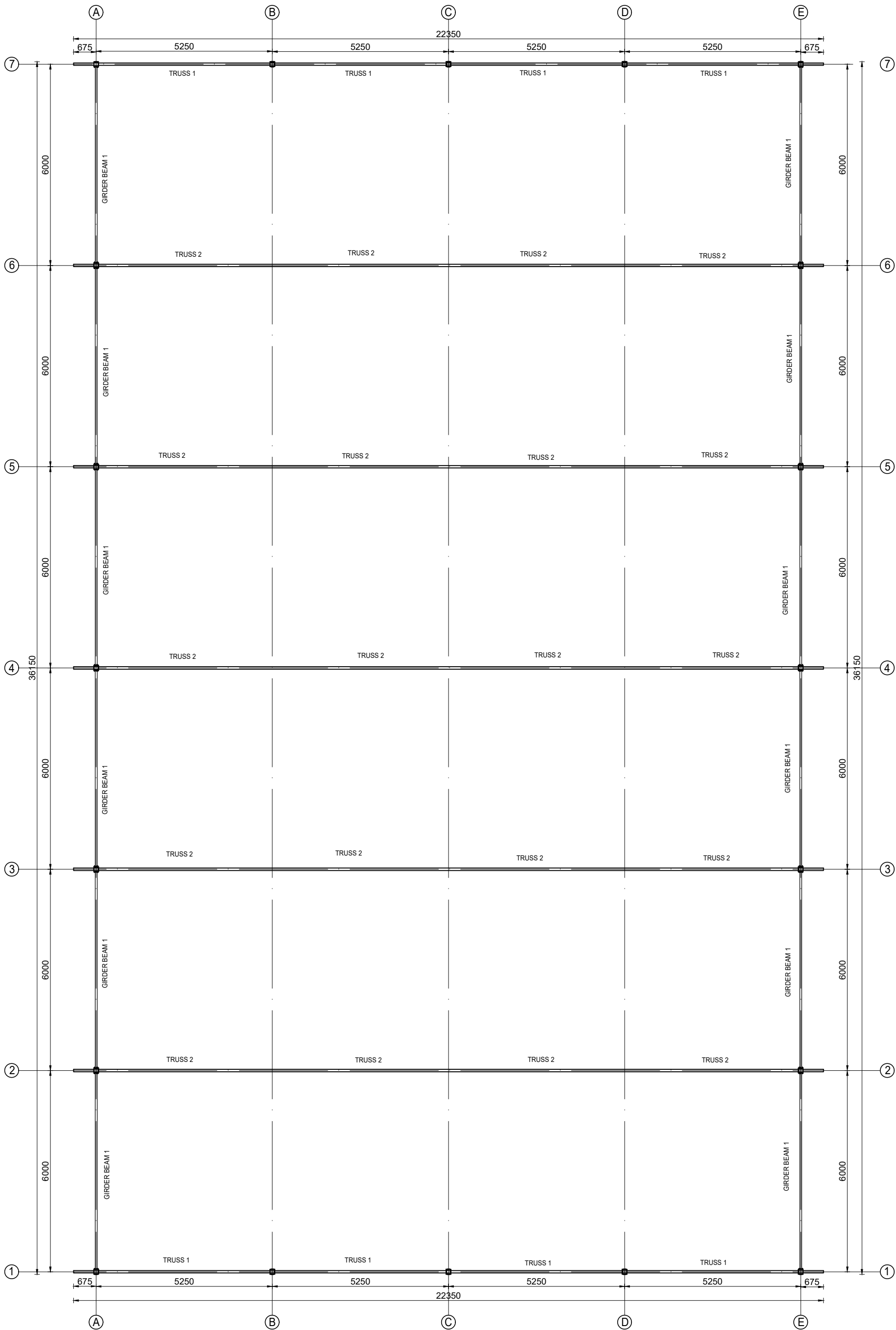
GIRDER BEAM AND TRUSS PLAN SCALE=1:100
