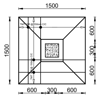
ISOLATED FOOTING PLAN SCALE=1:50
