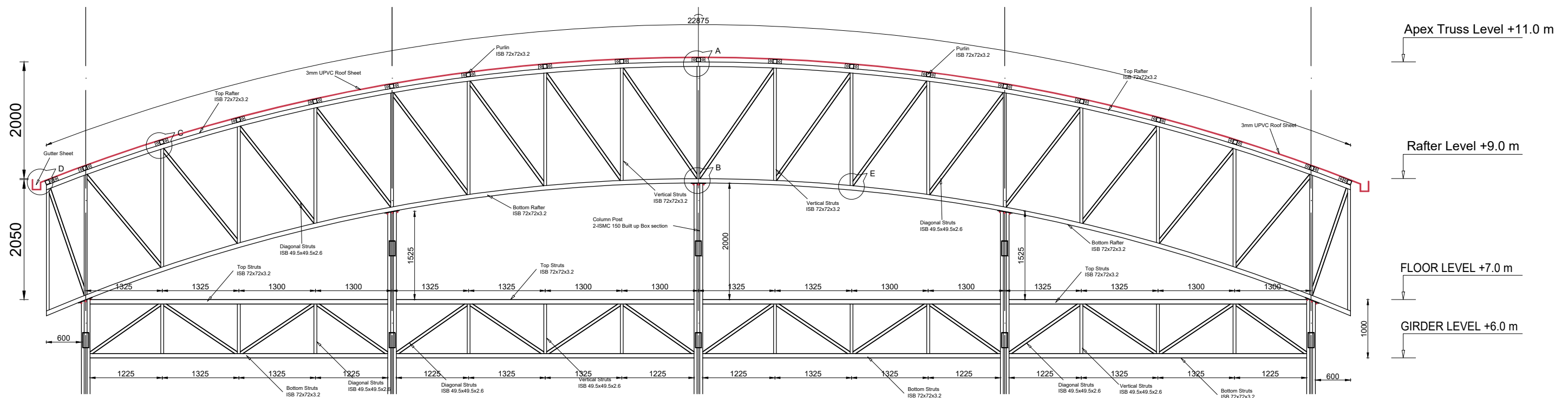
TRUSS PROFILE 1 SCALE=1:50
