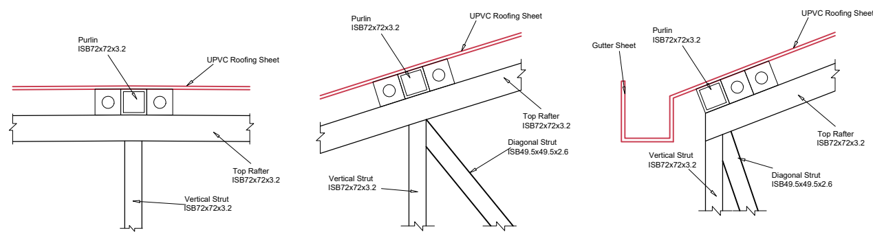
SECTIONAL DETAIL AT A
