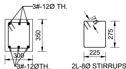
SECTION AT X1 Scale:=1:25
