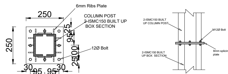
COLUMN SPLICING CONNECTION
