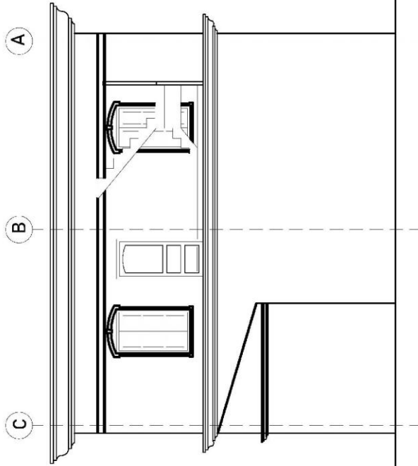
NORTH ELEVATION
