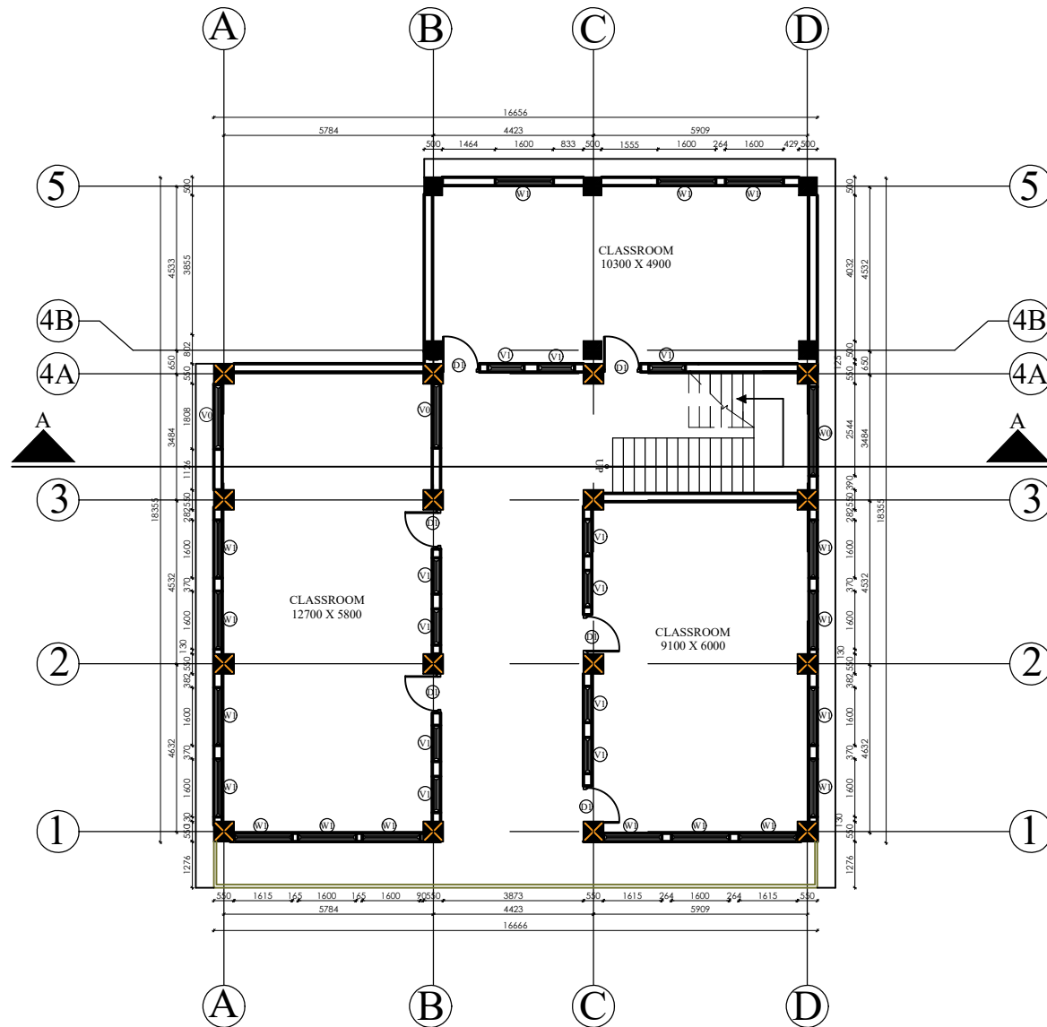
THIRD FLOOR PLAN AREA: 279.85 SQ. M
