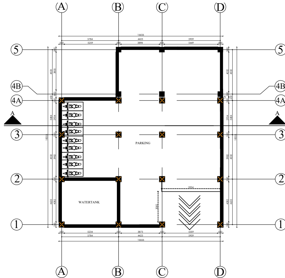
BASEMENT FLOOR PLAN AREA: 279.85 SQ. M
