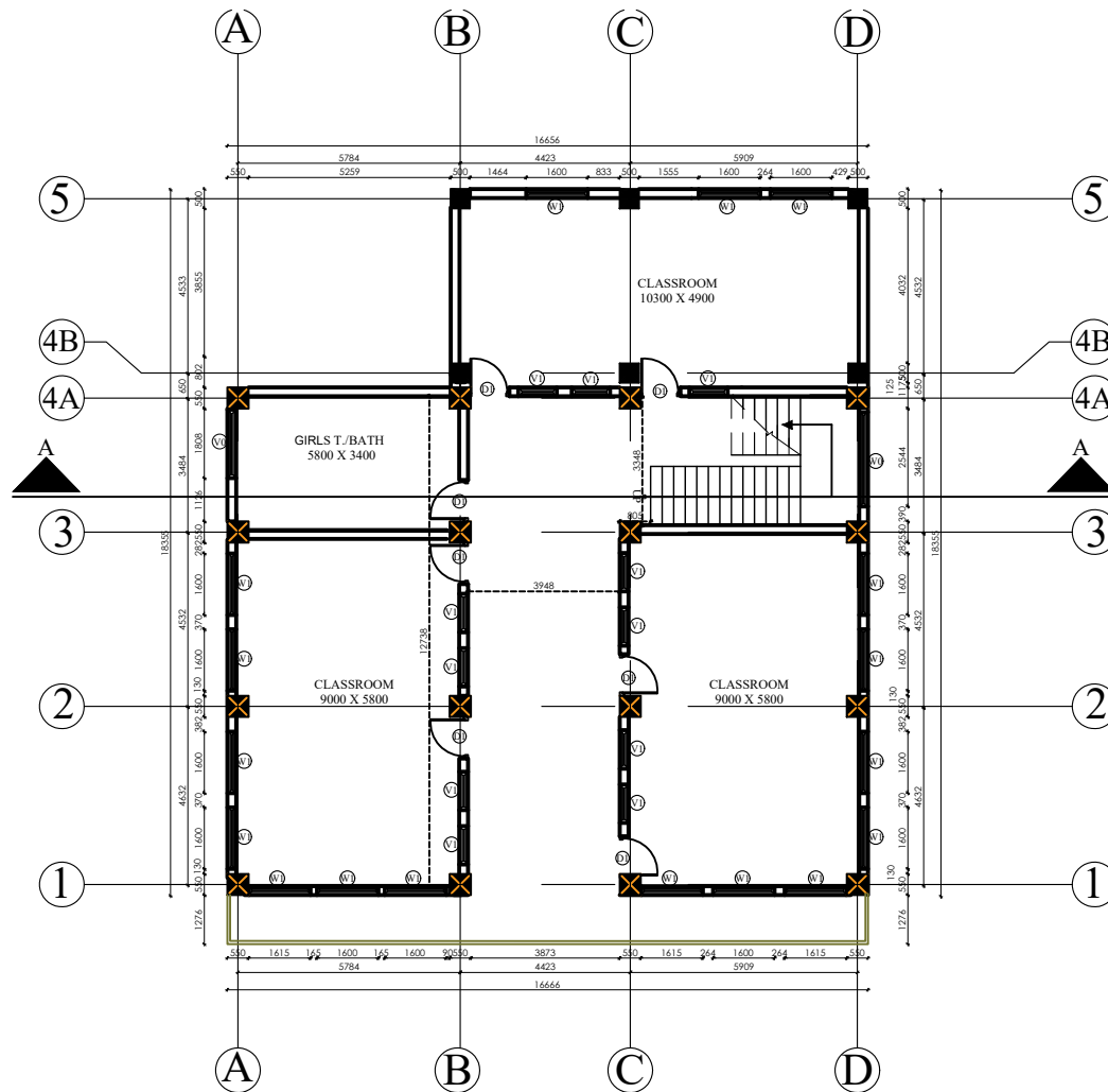
FIRST FLOOR PLAN AREA: 279.85 SQ. M
